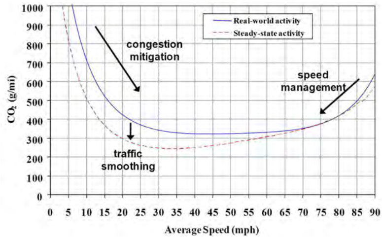
Figure 9 Relation between speed and CO 2 emissions for passenger cars, running on conventional oil-based fuels, with 3 different speed control measures. Note that the speed is in miles per hour (mph) [38].
