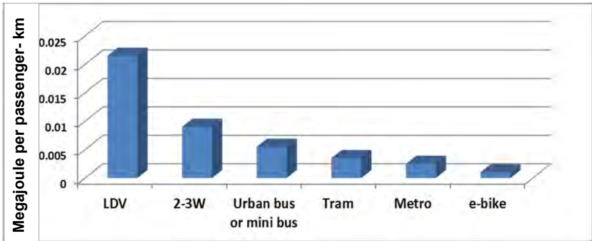
Figure 7 Comparison of energy efficiency for different mode of transport by passenger-kilometre based on Replege et al. 2014 EST conference [28]. LDV: Light Duty Vehicle
