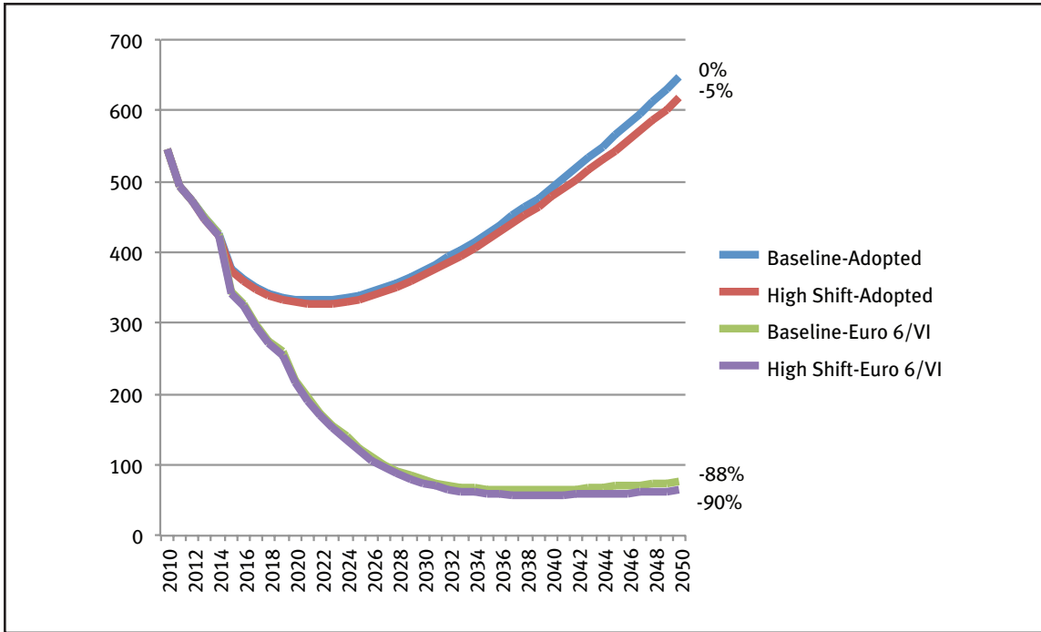
Figure 23 Global Primary PM2.5 Emissions from On-Road Vehicles in Urban Areas, 2010-2050
