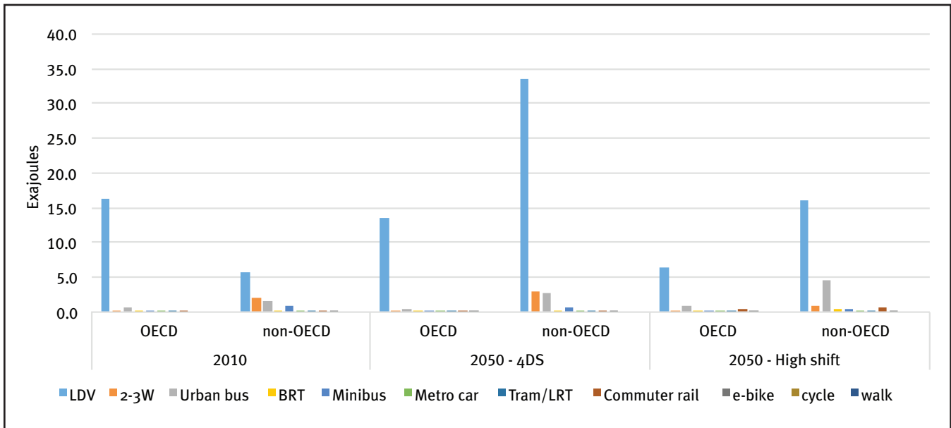
Figure 15: Energy Use by Scenario, Region, and Mode
