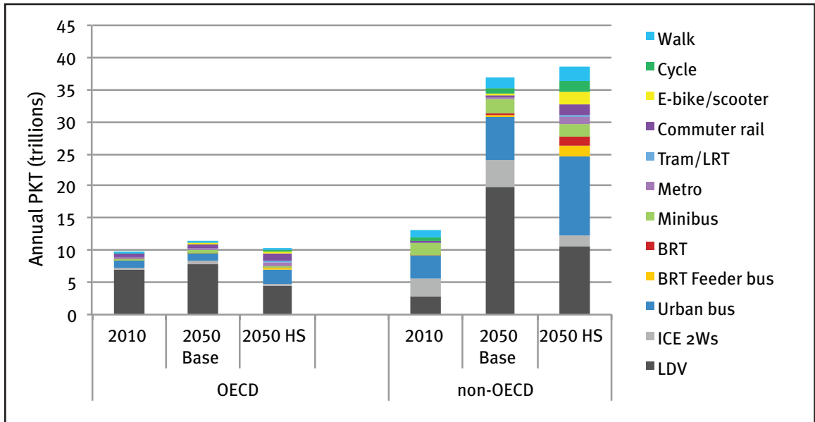
Figure 5: Total Passenger Kilometers of Urban Travel 2010, 2050 Base, and 2050 High Shift Scenario
