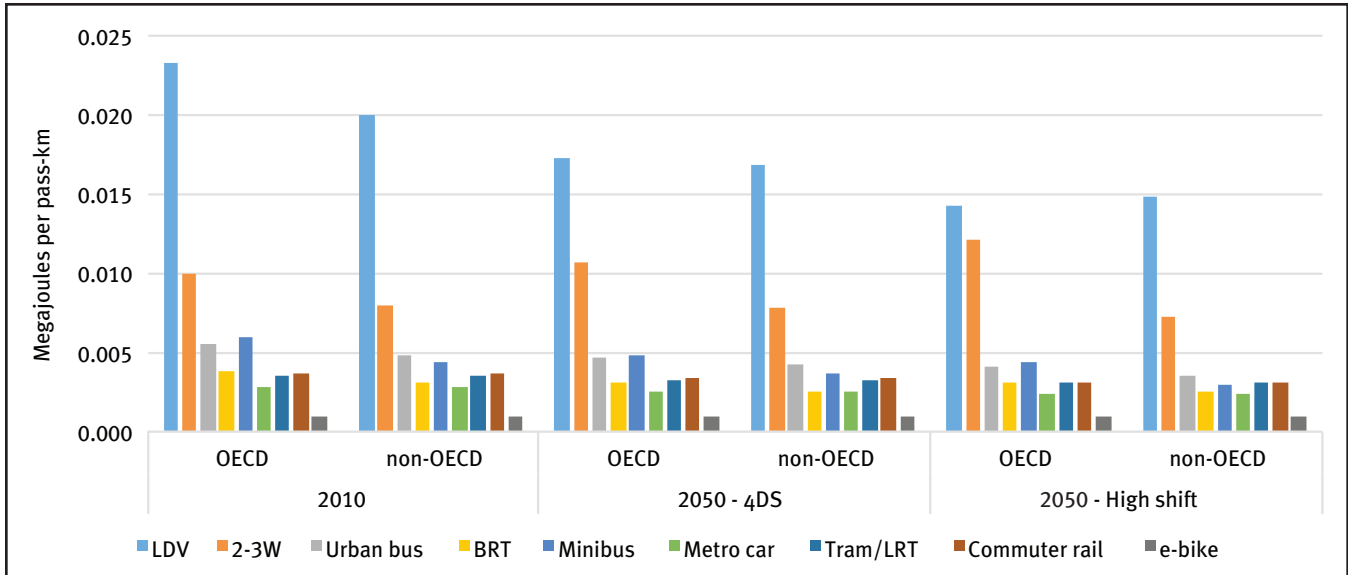
Figure 14: Energy Efficiency by Passenger-Kilometer By Mode by Year and Scenario
