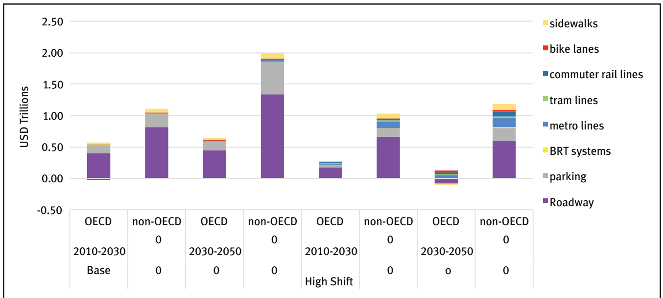
Figure 20: Infrastructure cost estimates, annual averages for 2010-2030 and 2030-2050 by type, scenario and mode
